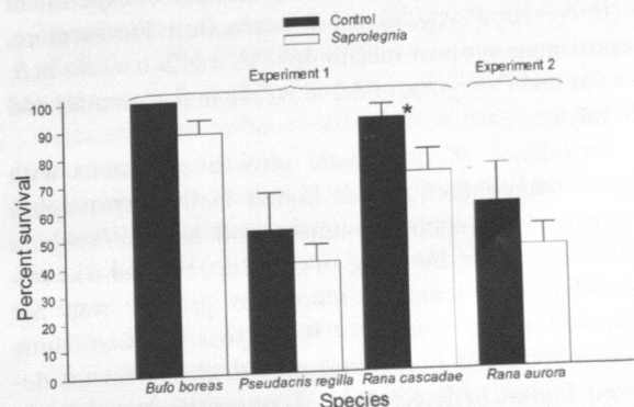
Fig. 1. Percent survival of metamorphs of Bufo boreas , Pseudacris regilla and Rana cascadae in experiment 1 and Rana aurora in experiment 2. Error bars are \pm 1 standard error. * Denotes the statistically significant difference between treatments for Rana cascadae .
